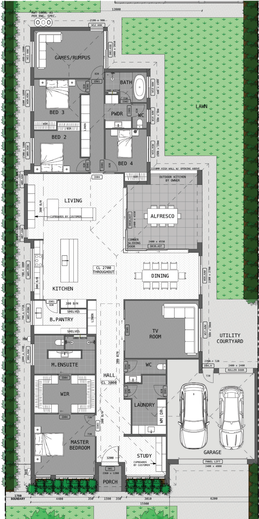
Ground Floor
