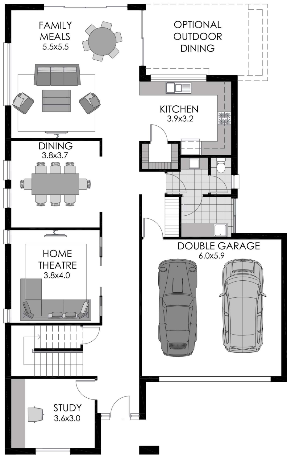
LOWER FLOOR
