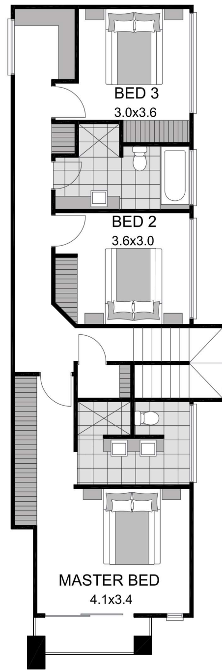
UPPER LEVEL
